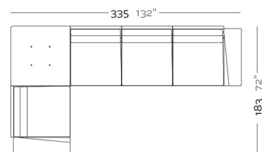
DELTA 4 Seats Sofa - Left DELTA Sofá 4 Plazas - Derecho
